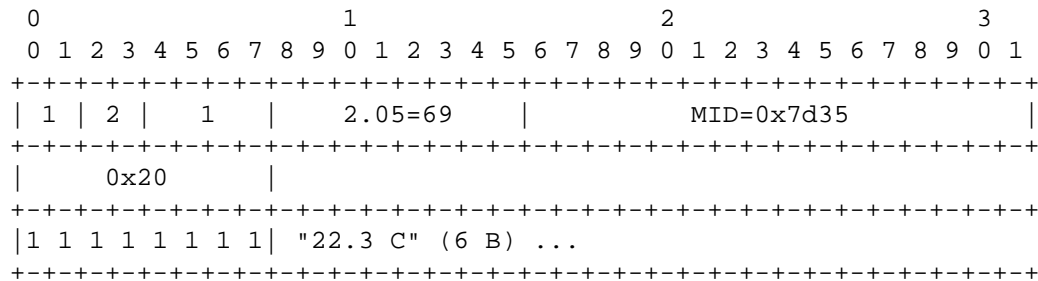
Figure 17: Confirmable Request; Piggybacked Response
