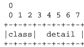
Figure 9: Structure of a Response Code
